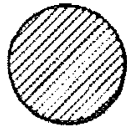
METAL NANOPARTICLE
