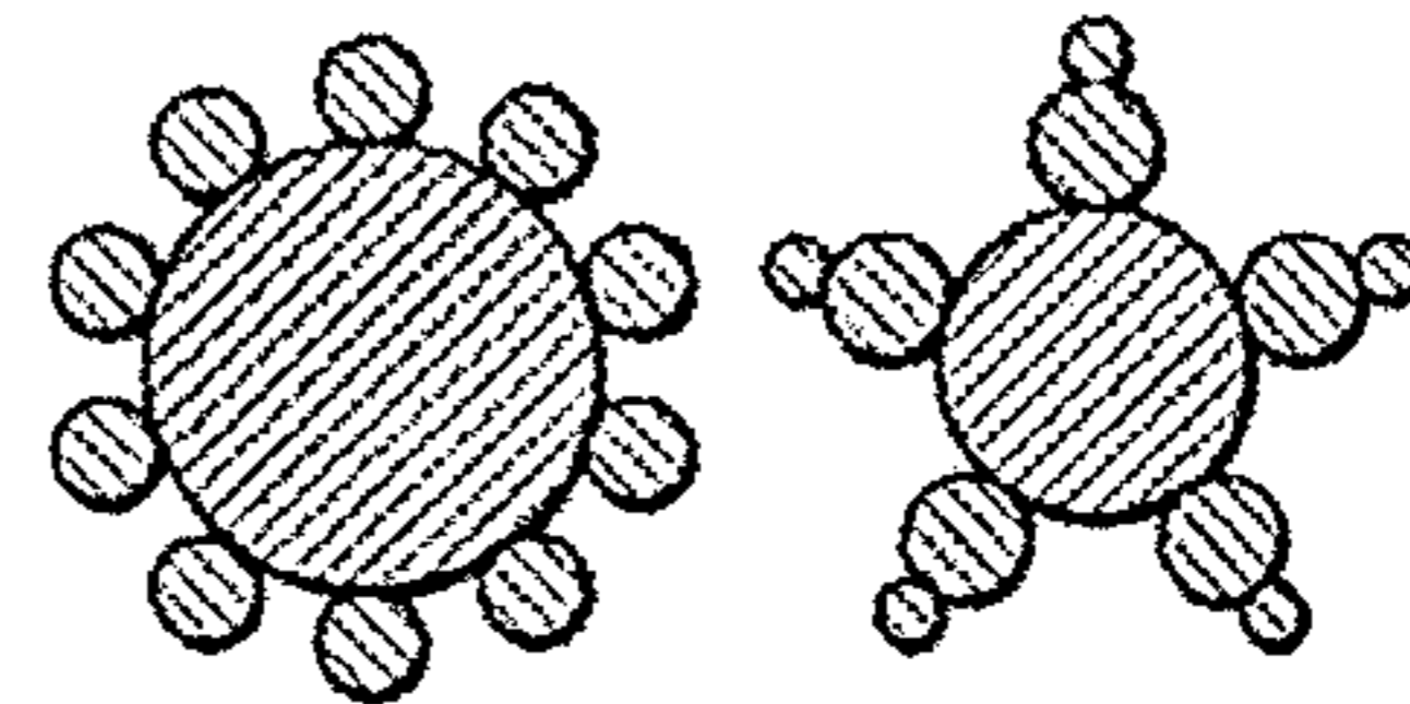
MULTI-NANOPARTICLE STRUCTURES
