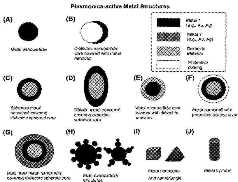
Figure 9. Plasmonics-active Nanostructures
