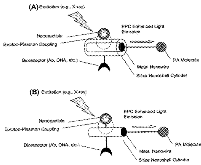
Exciton-Plasmon Coupling (EPC) Between Metal Nanorod and Nanoparticle
