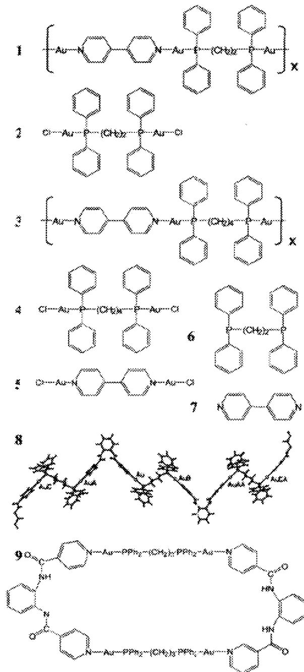
Figure 16. Gold complexes Exhibiting XEOL [Taken from : Kim et al, Inorg. Chem. , 46, 949, 2007].
