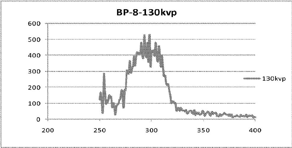
FIG. 2B LaF 3 :Ce having a measured emission at 300nm.
