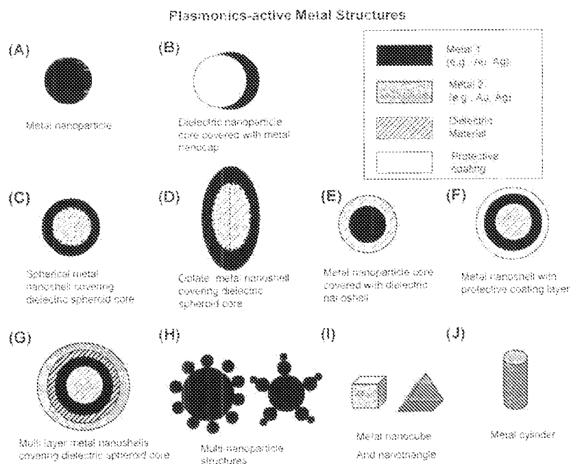
Figure 9. Plasmonics-active Nanostructures
