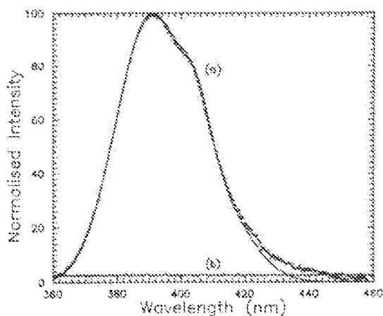
Figure 1. Curve a, the XEOL spectrum of BaFBr:Eu. The dotted curve is the observed spectrum and the continuous curve passing through the observed spectrum is the fitted spectrum. Curve b is the XEOL spectrum of pure BaFBr.
