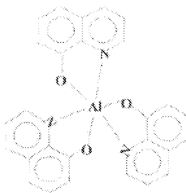
Figure 17. Tris 8-hydroxyquinoline –Aluminum Complex Exhibiting XEOL [Taken from: S. J. Naftel, P. Zhang, P.-S. Kim, and T. K. Sham, I. Coulthard, W. J. Antel, Jr., J. W. Freeland, and S. P. Frigo, M.-K. Fung and S. T. Lee, Y. F. Hu and B. W. Yates, Soft x-ray-excited luminescence and optical x-ray absorption fine structures of tris 8-hydroxyquinoline. Aluminum, Appl. Phys. Lett. , 78, 1844, 2001]
