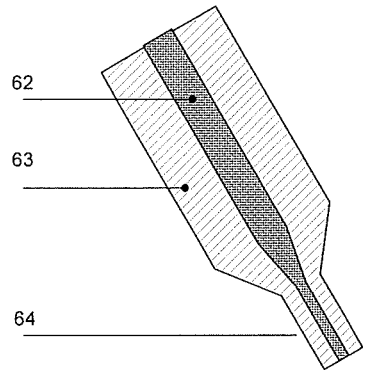
FIG. 33A - Dispensing of 2 adhesive beads
