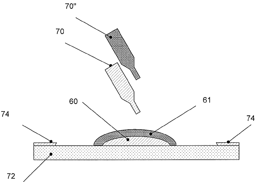
FIG. 33A - Dispensing of 2 adhesive beads
