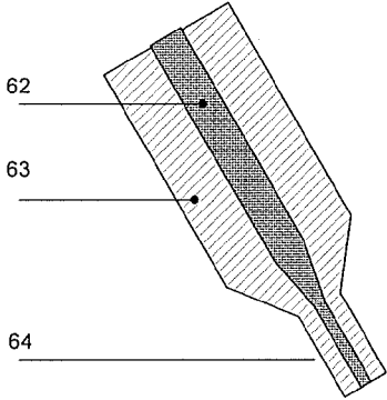
FIG. 33B - Special Dispensing syringe with 2 coaxial containers
