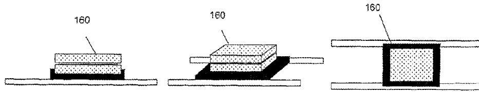
FIG. 40A- Different Perspective of the assemblies 160 interfacing with the conveyor.
