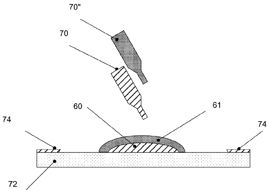
FIG. 33A - Dispensing of 2 adhesive beads
