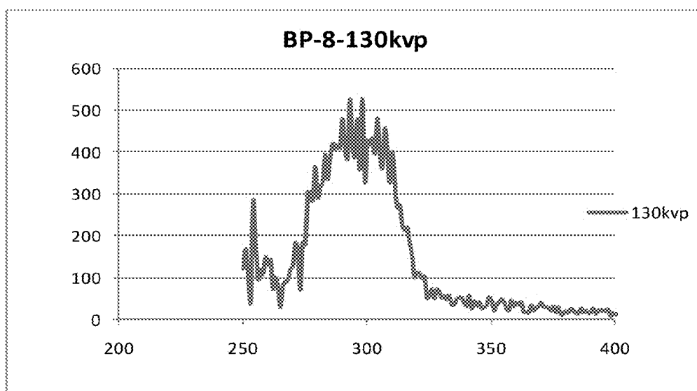
FIG. 2. \text{LaF}_3:\text{Ce} was reported to emit at 280nm under X-ray and was measured during the course of the present invention to emit at 300nm.
