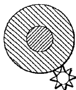
PA MOLECULES BOUND TO METAL NANOPARTICLE
