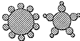
MULTI-NANOPARTICLE STRUCTURES
