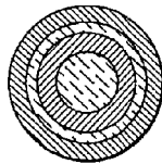
MULTI-LAYER METAL NANOSHELLS COVERING DIELECTRIC SPHEROID CORE
