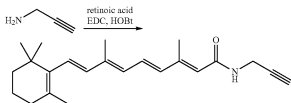
(2E,4E,6E,8E)-3,7-Dimethyl-N-(prop-2-ynyl)-9-(2,6,6-trimethylcyclohex-1-enyl)nona-2,4,6,8-tetraenamide
