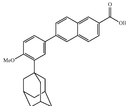
6-(3-(1-Adamantyl)-4-(methoxyphenyl)-2-naphthoic acid
