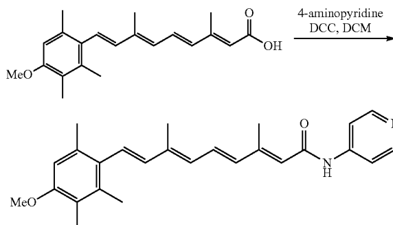
(2E,4E,6E,8E)-9-(4-Methoxy-2,3,6-trimethylphenyl)-3,7-dimethyl-N-(pyridin-4-yl)nona-2,4,6,8-tetraenamido
