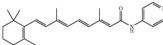
(2E,4E,6E,8E)-3,7-dimethyl-N-(pyridin-4-yl)-9-(2,6,6-trimethylcyclohex-1-enyl)nona-2,4,6,8-tetraenamide
