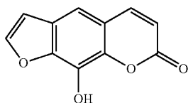
8-Hydroxypsoralen
