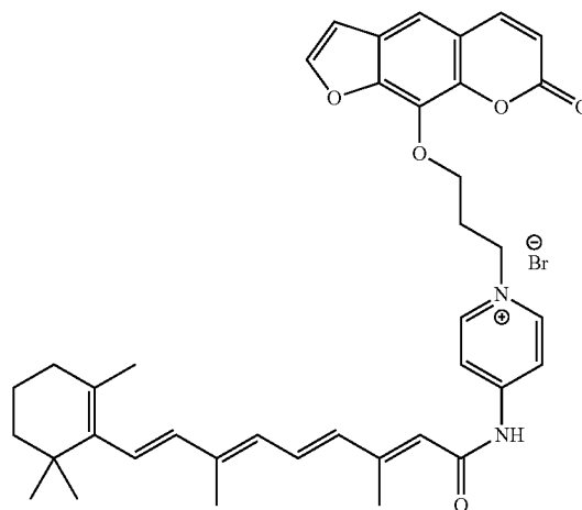
psoralen derivative
