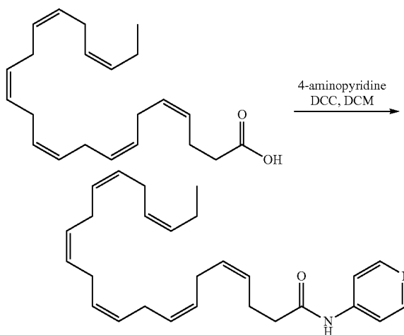
(4Z,7Z,10Z,13Z,16Z,19Z)-N-(Pyridin-4-yl)docosa-4,7,10,13,16,19-hexaenamide
