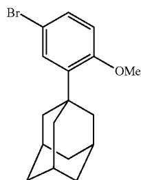
2-(1-Adamantyl)-4-bromoanisole
