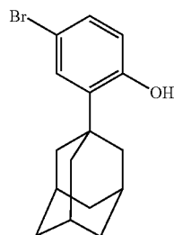
2-(1-Adamantyl)-4-bromophenol
