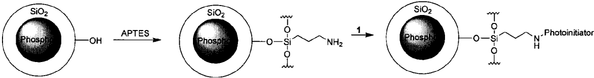
Irgacure 2959 photoinitiator activated ester
