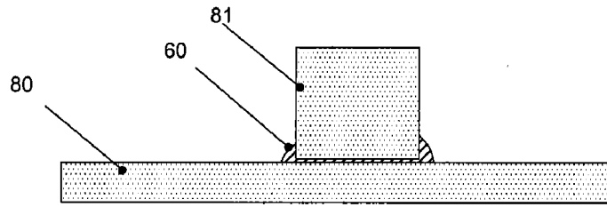
FIG. 31A - Adhesive dispense on composite substrate
