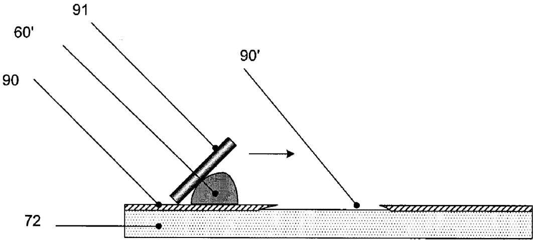
FIG. 30A - Alignment prior to screen printing
