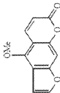
5-Methoxypsoralen (5-MOP)
