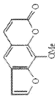
8-Methoxypsoralen (8-MOP)
