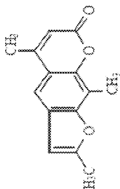
4,5,8-Trimethoxypsoralen (TMP)
