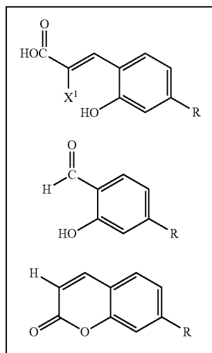
X^1 = \text{H or Br}
