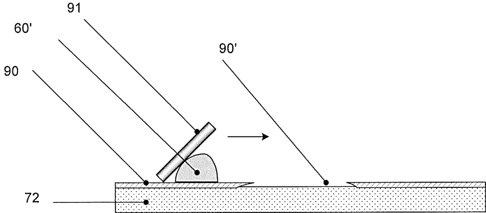
FIG. 30A - Alignment prior to screen printing
