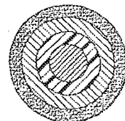
X-RAY CONVERTER NANOPARTICLE COVERED WITH DIELECTRIC LAYER AND METAL NANOSHELL WITH PROTECTIVE COATING LAYER
