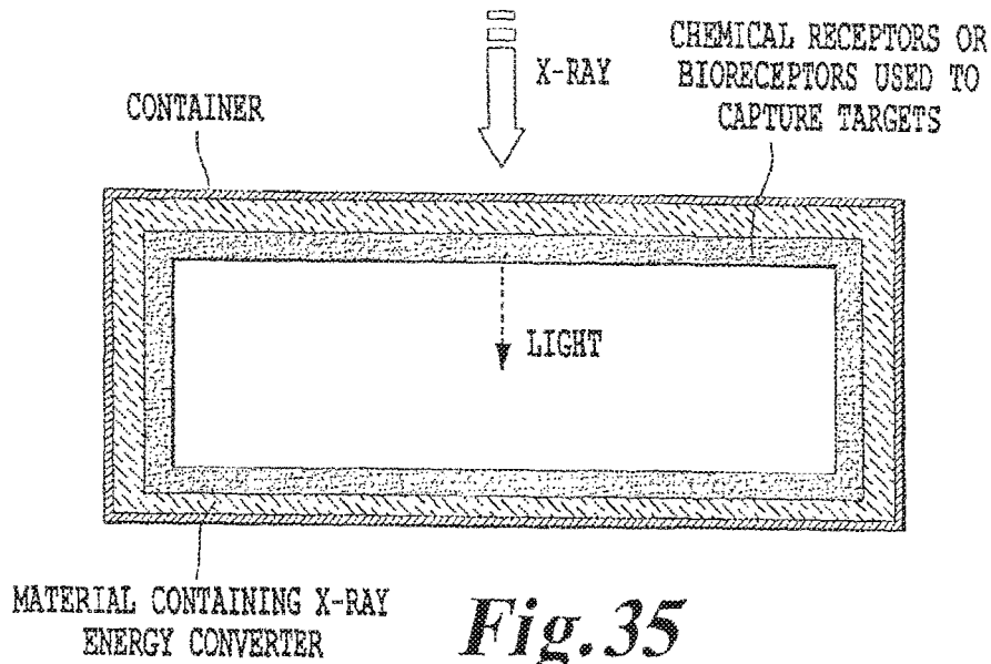
STERILIZATION SYSTEM 9 WITH CHEMICAL RECEPTORS OR BIORECEPTORS
