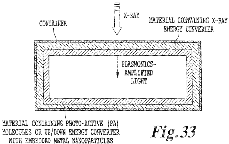
STERILIZATION SYSTEM 7 WITH PLASMONICS
