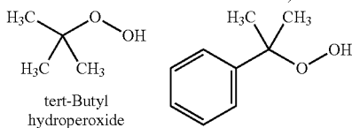
Cumene hydroperoxide
