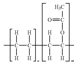
Ethylene-vinyl acetate
