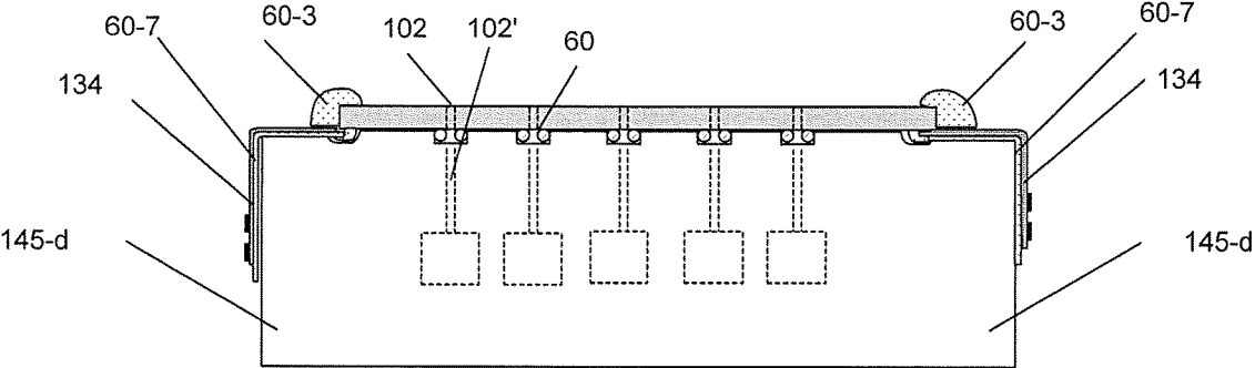
FIG. 55B The flex is adhered to the external walls of the fluidic reservoirs.
